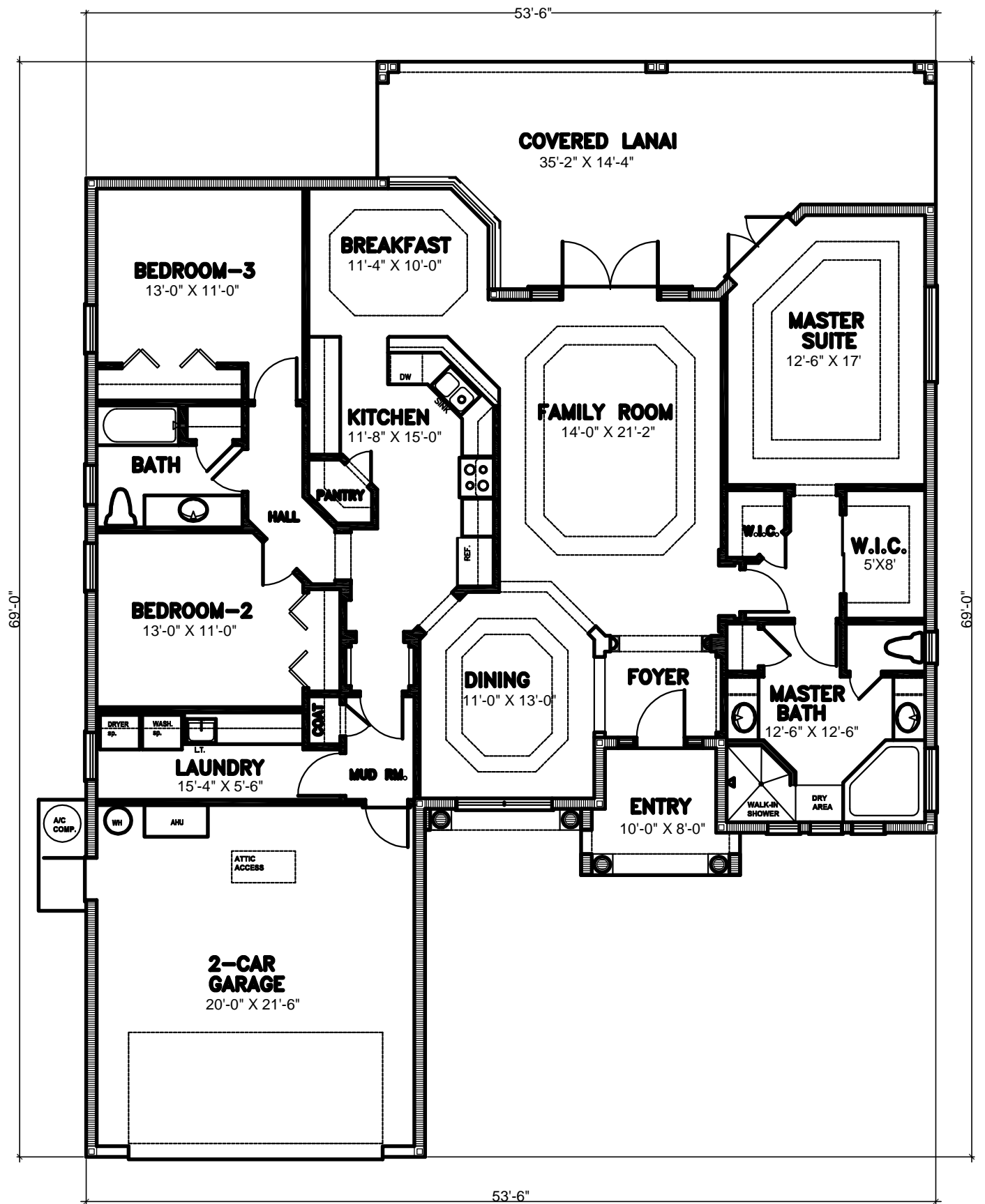
FLOOR PLAN
