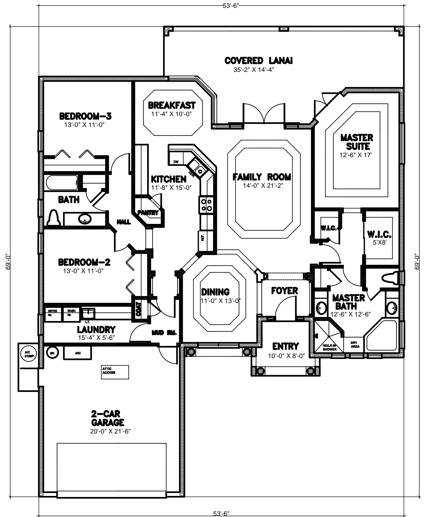
FLOOR PLAN
